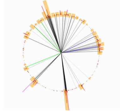
Fig. 3: Event display of a high-multiplicity state arising from the process in Fig. 2, in a model where the v -hadrons decay mainly to b\bar{b} pairs.
