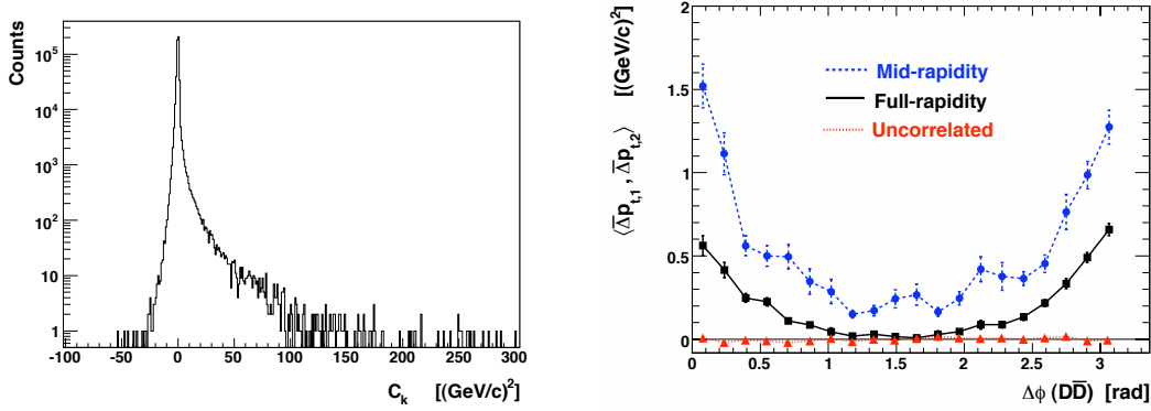
Fig. 2: (Colour online) Distribution of the p_t convariance C_k for D\bar{D} pairs from p-p collisions at \sqrt{s} = 14 TeV as calculated by PYTHIA (v. 6.406) (left panel) and their momentum correlator \langle \Delta p_{t,1}, \Delta p_{t,2} \rangle as a function of \Delta\phi at full rapidity, mid-rapidity and for background using the mixed event method (right panel).
