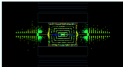
Figure 7 : The inner detector part of SiD. WIRE4 event display of the pair background of one bunch crossing.
