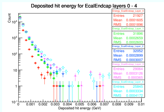
Figure 11 : Energy distribution of the hits in the first five layers of the SiD EcalEndcaps
