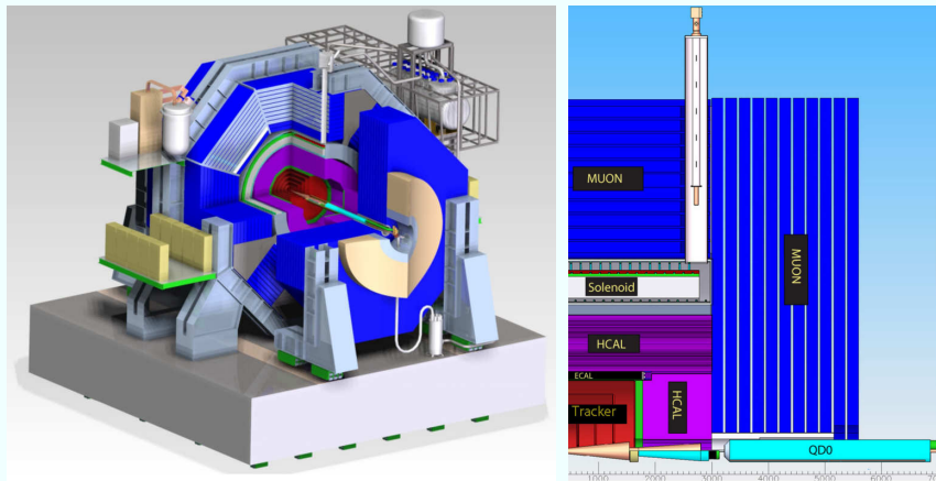
Figure 1 : SiD detector model: Vertex detector (red), ECAL (green), HCAL (pink), Muon system (blue)
