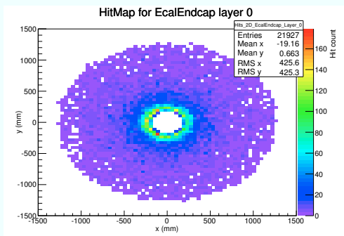
Figure 8 : 2D hit map of the hits from a full pair background train in the EcalEndcap layer 0.
