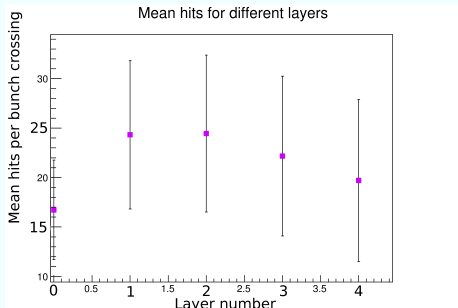
Figure 4 : Comparison of the MEAN number of hits in the first 5 layers of the EcalEndcaps.
