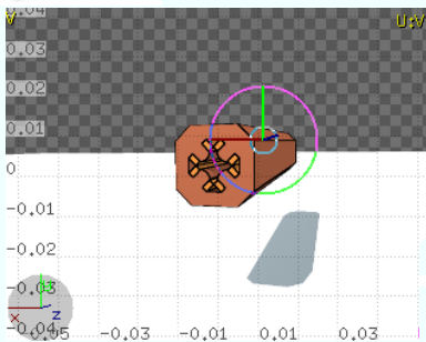
Figure 6 : FLUKA simulation model of one of the ILC lattice quadrupoles.
