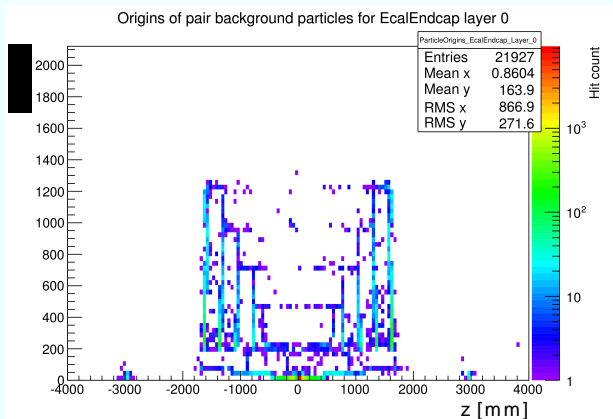
Figure 5 : 2D map of the origins of the pair background particles that hit the EcalEndcap layer 0.
