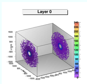
Figure 9 : 3D hit map of the hits from a full pair background train in the EcalEndcap layer 0.
