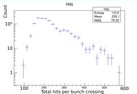
Figure 3 : Hits of pair background particles from a full train in the EcalEndcaps
