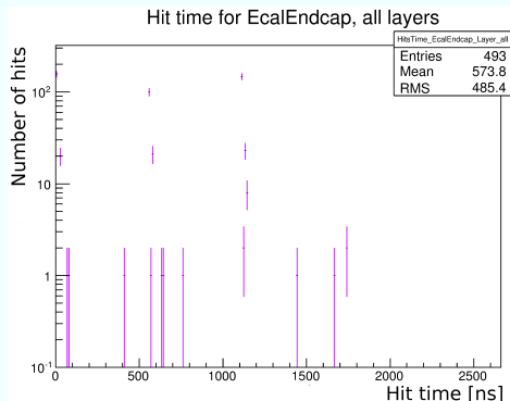
Figure 10 : Number of particles arriving at the EcalEndcaps as a function of the absolute time.
