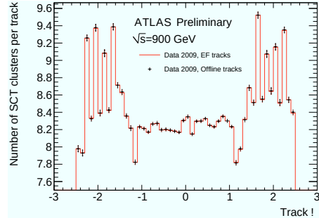
Figure 2: Average number of SCT hits per EF track (data and offline).
