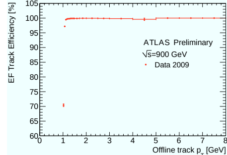
Figure 4: EF tracking efficiency vs p_T w.r.t. offline (data).
