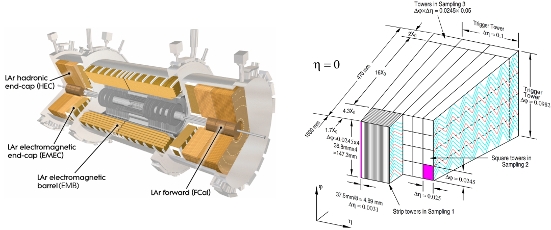
Figure 1: Schematic view of the liquid argon calorimeter system.
