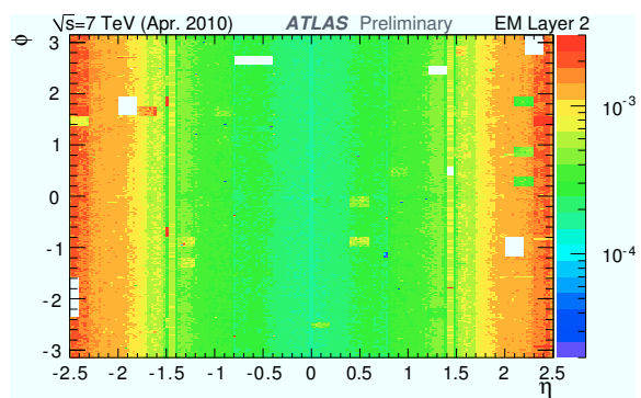
Figure 6: Cell occupancy map in the EM calorimeter with 7 TeV collision data.
