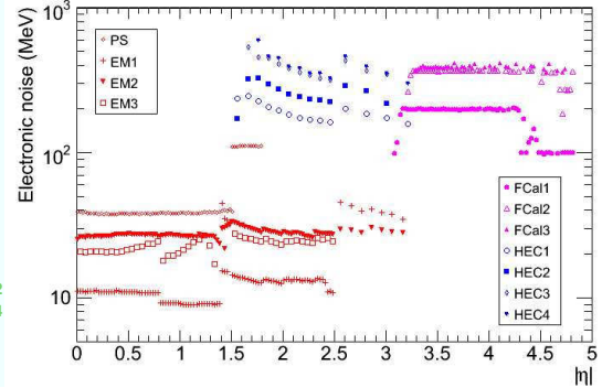
Figure 4: Electronic noise at cell level as a function of |\eta| for each longitudinal layer of the calorimeter.
