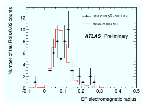
Figure 1: Candidate \tau jet EM radius distribution at EF. Dots are 2009 collision data, solid line is MC expectation.
