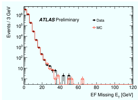
Figure 4: Distribution of missing E_T at EF. Dots are 7 TeV collision data, solid line is MC expectation.
