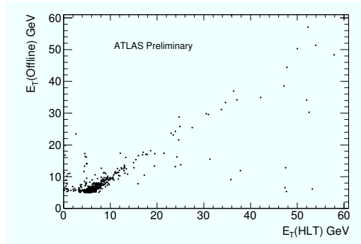
Figure 5: Correlation of the EF and offline E_T obtained from 900 GeV data.
