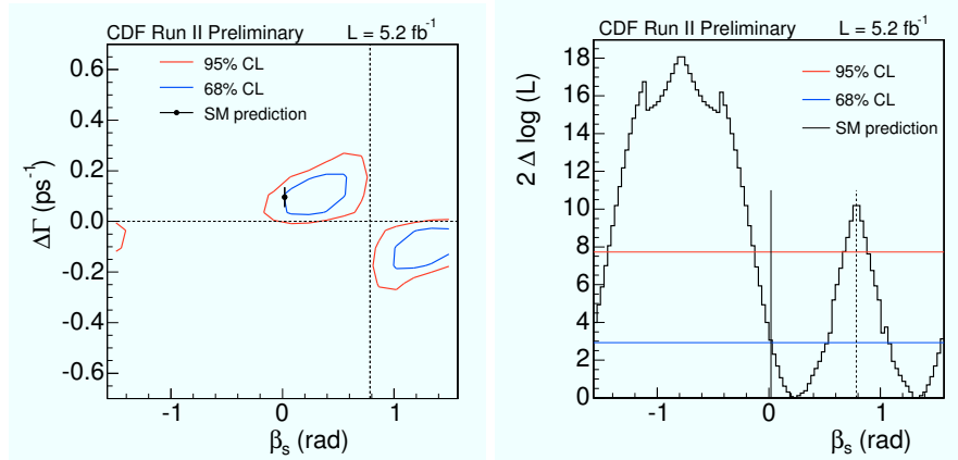
Figure 3: Confidence regions in the \beta_s - \Delta\Gamma plane (left) and \beta_s (right).
