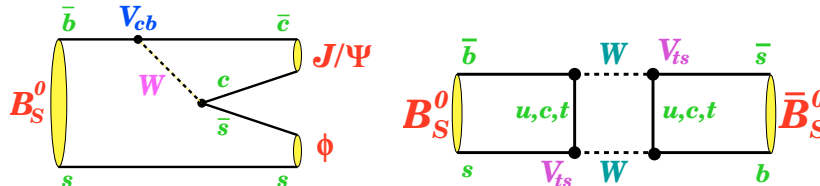
Figure 1: The B_s^0 meson can decay to J/\psi\phi directly (left), or can mix to a \bar{B}_s^0 meson before decaying (right).
