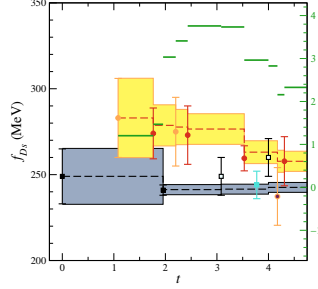
Figure 3: Comparison of the predicted f_{D_s} with experimental results. The circles denote experimental values with the yellow band showing the average. The squares show the prediction and the gray area the theory average. The green lines denote the difference between theory and experiment in Gaussian \sigma . The time t is measured in years since June 2005.
