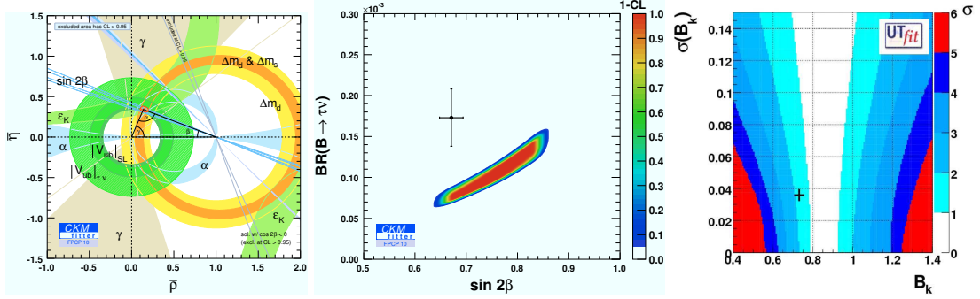
Figure 7: The global status of the unitarity triangle fit from the CKMfitter group (left), the graphical representation of the B \rightarrow \tau \nu versus \sin 2\beta disagreement (middle) and the situation with indirect and direct determinations of the parameter proportional to \epsilon_K from the UTFit group (right). In the middle plot, colored confidence regions show the expectation for the B \rightarrow \tau \nu branching fraction from the fit where two quantities are excluded while the point shows experimental results. In the right plot, the colored areas show the confidence regions of B_K from the fit without constraint from the CP -violation in the kaon system. The cross represents the experimental measurement of the quantity.
