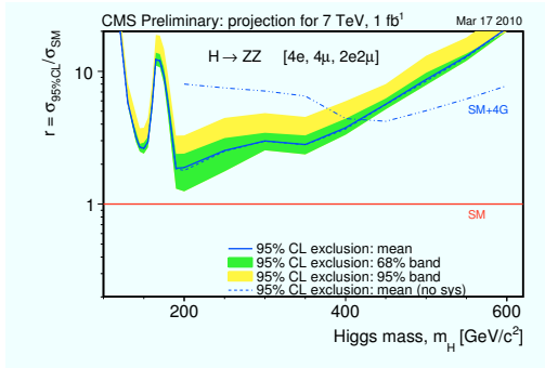
Figure 3: Exclusion plot for the H \rightarrow ZZ \rightarrow 4\ell channel, for \sqrt{s} = 7 \text{ TeV} and L = 1 \text{ fb}^{-1} .
