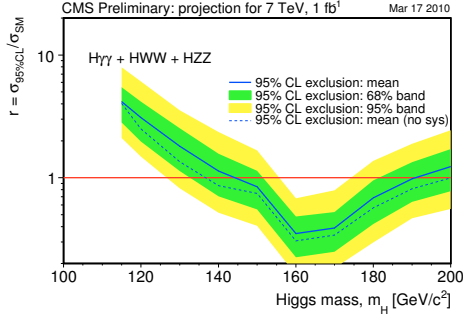
Figure 5: Expected exclusion limits for the combination of the channels, assuming absence of signal, for \sqrt{s} = 7 \text{ TeV} and L = 1 \text{ fb}^{-1} .
