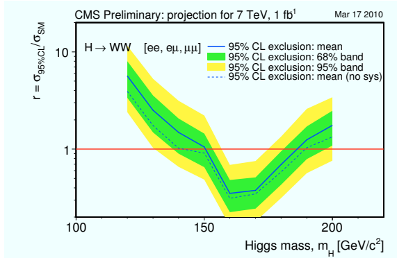
Figure 1: Exclusion plot for the H \rightarrow WW \rightarrow 2\ell 2\nu channel, for \sqrt{s} = 7 TeV and L = 1 fb ^{-1} , assuming absence of signal.
