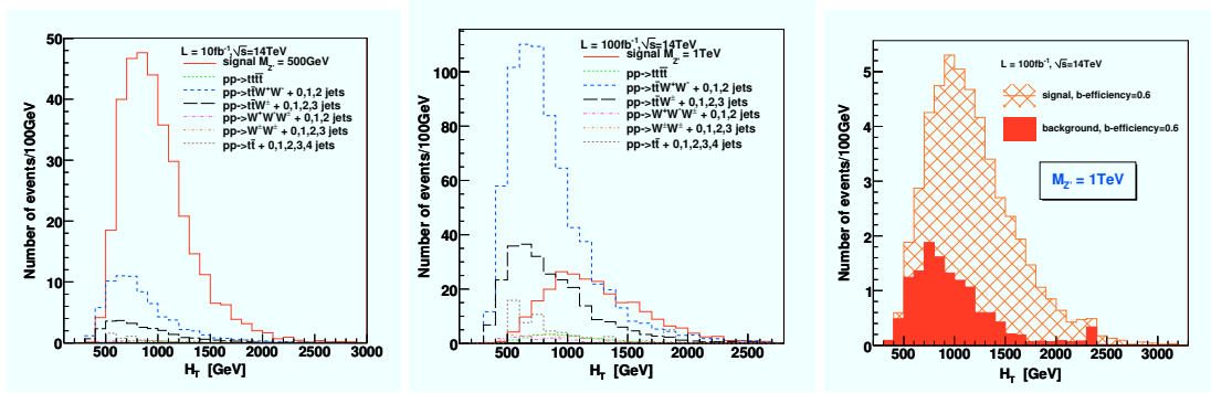
Figure 5: Total transverse energy after demanding n_j \geq 6 , p_T > 30 GeV (first two plots) and in addition n_{b-jet} \geq 3 (third plot). In first plot, M_{Z'} = 500 GeV, in last two plots M_{Z'} = 1 TeV.
