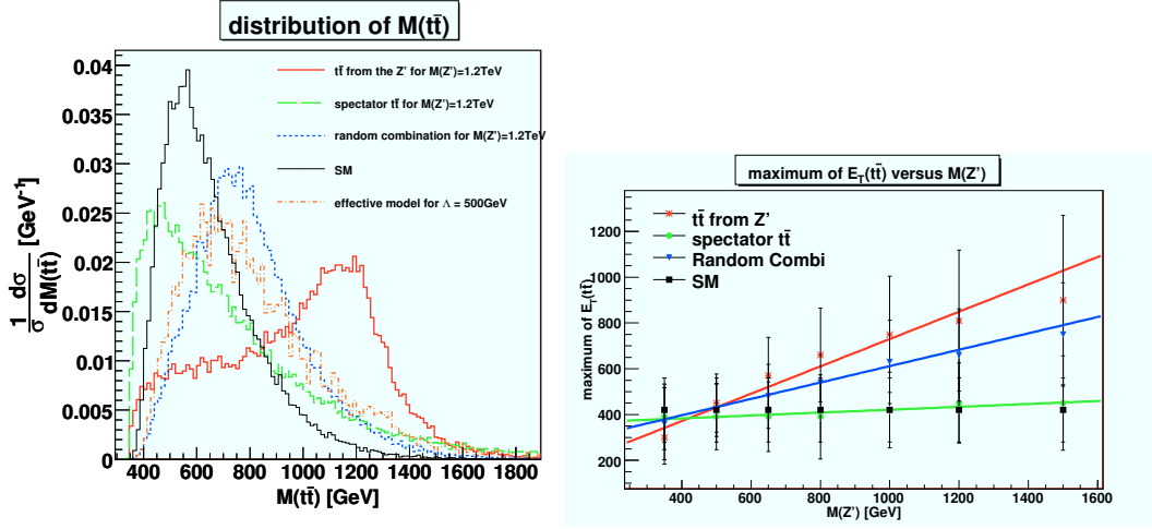
Figure 3: (a) Invariant mass distributions of the top pairs; (b) Position of the maximum of the E_T distribution of the t\bar{t} pair as a function of M_{Z'} .
