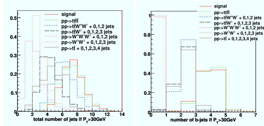
Figure 4: Fractions of signal and background events with a given number of jets with p_T > 30 GeV in the same-sign dilepton channel, after Pythia and jet reconstruction with a jet cone size \Delta R = 0.4 .
