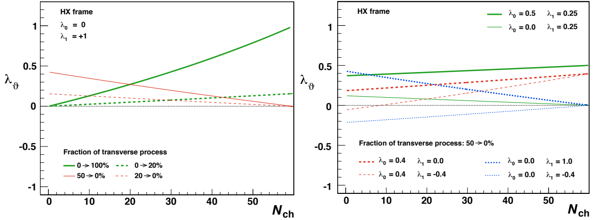
Figure 6: Expected N_{ch} -dependences of the \lambda_\theta parameter for the sum of two processes, of polarizations \lambda_0 and \lambda_1 , of relative fractions changing linearly with N_{ch} (see text for details).
