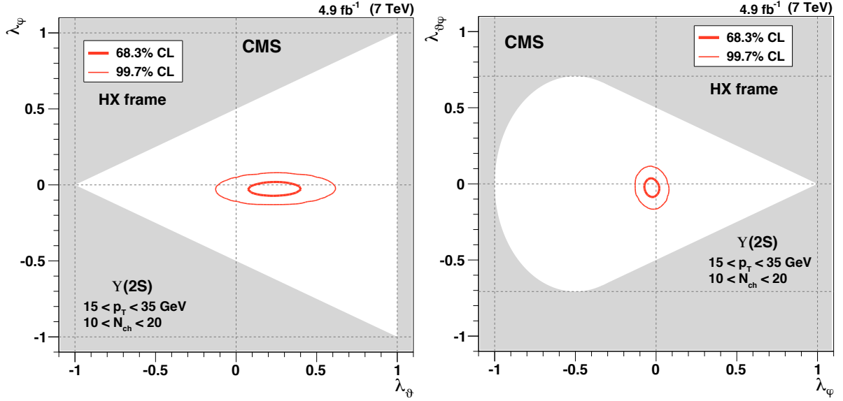
Figure 4: Two-dimensional marginals of the PPD for the HX frame in the \lambda_\theta vs. \lambda_\phi (left) and \lambda_{\theta\phi} vs. \lambda_\phi (right) planes, for Y(2S) with 15 < p_T < 35 GeV and 10 < N_{\text{ch}} < 20 , displaying the 68.3% and 99.7% CL total uncertainties. The shaded areas represent physically forbidden regions of parameter space for the decay of a J = 1 particle [14].
