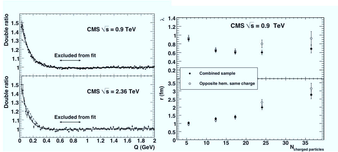
Figure 2: (Left) Fits to the double ratios \mathcal{R}^{\text{comb}}(Q) with exponential (solid lines) and Gaussian (dashed lines) functions, for 0.9 TeV (top) and 2.36 TeV (bottom) data. The range 0.6 < Q < 0.9 GeV is excluded from the fits. (Right) Values of the \lambda (top) and r (bottom) parameters as a function of the charged-particle multiplicity for combined (dots) and opposite-hemisphere, same-charge (open circles) reference samples, at 0.9 TeV. The errors shown are statistical only.
