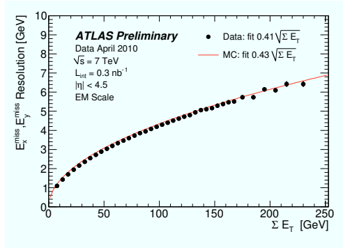
Figure 3: The E_x^{\text{miss}} , E_y^{\text{miss}} resolutions as a function of the \sum E_T for data and Monte Carlo simulation.
