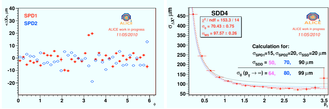
Figure 1: Mean values of the "unbiased" local residual distributions for SPD modules (left panel) and widths of the "unbiased" local residual distributions for SDD modules in layer 4 (right panel) – see text for details.
