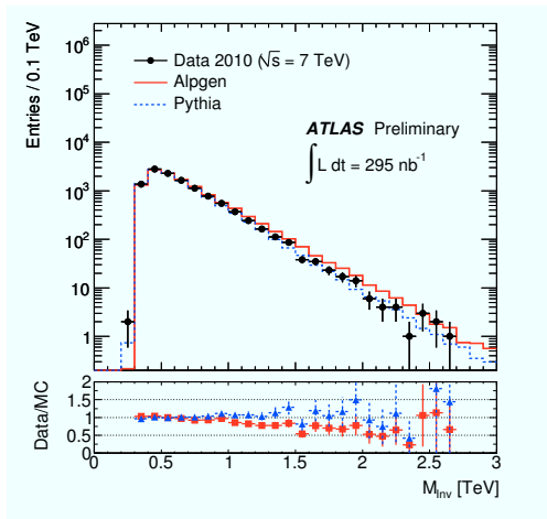
Figure 1: Invariant mass distribution for events with at least three objects and with \sum p_T > 300 GeV after normalising the background to data. The solid dots are the data, while the solid and dashed histograms are the background predictions using scaled Alpgen and Pythia, respectively.
