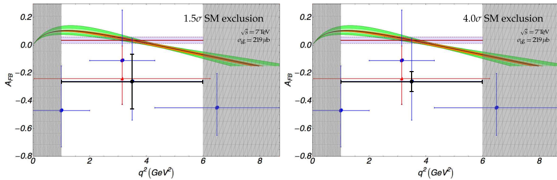
Figure 2: Precision with which A_{FB} can be determined at LHCb from 0.1 \text{ fb}^{-1} (left) and 1 \text{ fb}^{-1} of data. The SM prediction is shown as a line surrounded by a grey area (theoretical uncertainty). The blue (dark grey) ellipses correspond to the Belle measurement, the red (light grey) triangle to the Babar measurement and the black circle is the LHCb expectation assuming the Belle A_{FB} central value in the region from 1 to 6 \text{GeV}^2 .
