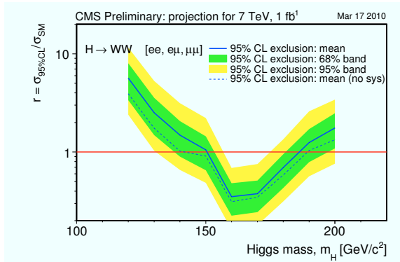
Figure 1: Exclusion plot for the H \rightarrow WW \rightarrow 2\ell 2\nu channel, for \sqrt{s} = 7 TeV and L = 1 fb ^{-1} , assuming absence of signal.
