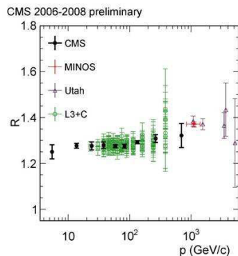
Figure 4: Flux ratio of positive to negative muons in cosmic-rays.
