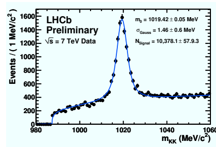
Figure 4: \phi \rightarrow K^+K^- selection using RICH detectors
