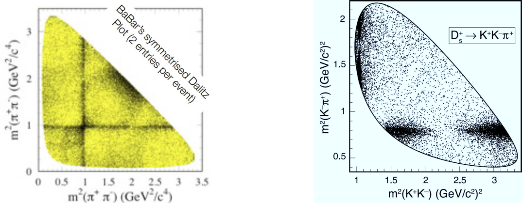
Figure 2: Dalitz distributions for three-body decays of the D meson.
