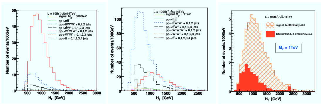
Figure 5: Total transverse energy after demanding n_j \geq 6 , p_T > 30 GeV (first two plots) and in addition n_{b\text{-jet}} \geq 3 (third plot). In first plot, M_{Z'} = 500 GeV, in last two plots M_{Z'} = 1 TeV.
