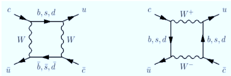
Figure 3: Quark level diagrams for D^0-\bar{D}^0 mixing
