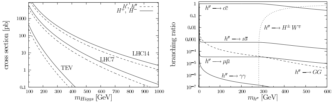
Figure 2: left: total cross section of Drell–Yan type Higgs boson production at TEVATRON and LHC. right: branching ratios of the CP odd h'' Higgs boson, where a mass of m_{H^\pm} = 200 GeV is assumed.
