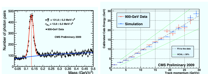
Figure 2: Left: photon-pair invariant-mass distribution in the barrel ( |\eta| < 1.0 ) for the data. Right: average calibrated calorimeter response as a function of the track momentum for the 900 GeV data (light upwards triangles) and for the simulation (dark downwards triangles). The dashed lines show the same quantity when the HCAL raw response is changed by \pm 30\%
