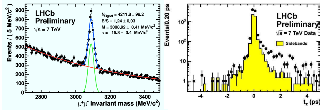
Figure 5: Left: Dimuon invariant mass distribution showing the J/\psi \rightarrow \mu^+\mu^- signal in \sim 14 \text{ nb}^{-1} of data at \sqrt{s} = 7 \text{ TeV} . Right: Pseudo-proper time distribution of the J/\psi candidates in the signal window (black points) and in the sidebands (yellow histogram). The difference between the two distributions corresponds to signal J/\psi and displays a tail at large proper time indicative of b \rightarrow J/\psi X production.
