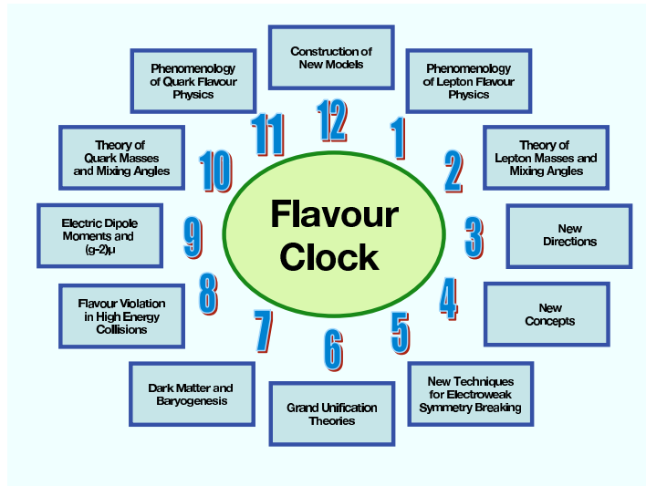
Figure 1: Working towards the Theory of Flavour around the Flavour Clock.
