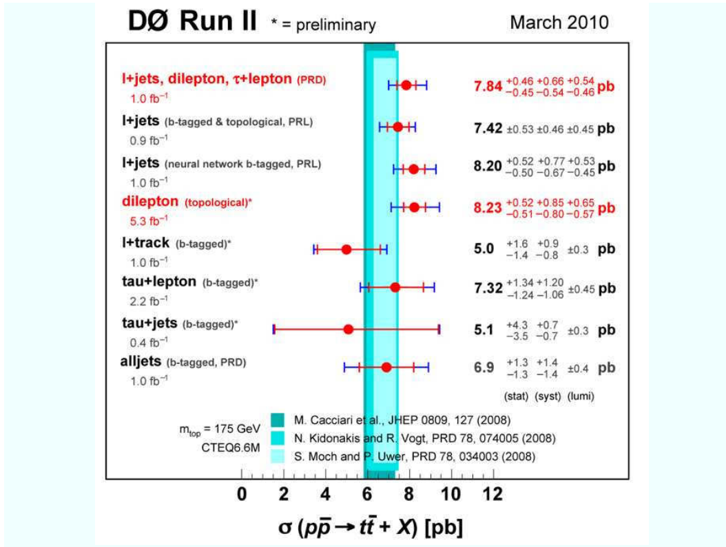
Figure 1: Recent measurements of the top quark pair production cross section at D0, in lepton+jets, dilepton and hadronic channels.
