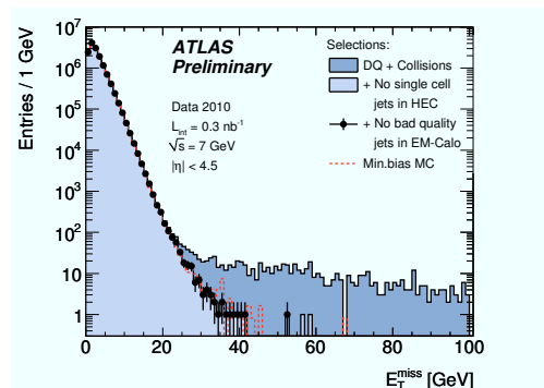
Figure 1: E_T^{\text{miss}} distribution for collision events from 7 TeV data, after successive selections. The corresponding distribution from Monte Carlo simulation is overlaid.
