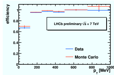
Figure 5: Tracking efficiency vs p_T of K_S
