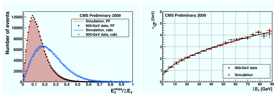
Figure 4: Left: distribution of the particle-based (solid) and calorimeter-based (hollow) E_T^{\text{miss}}/\Sigma E_T in the data (dots) and in the simulation (histogram). Right: resolution of the particle-based E_{x,y}^{\text{miss}} as a function of the particle-based in the data (dots) and in the simulation (squares).
