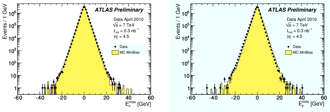
Figure 2: E_x^{\text{miss}} and E_y^{\text{miss}} distributions for data and Monte Carlo simulation.
