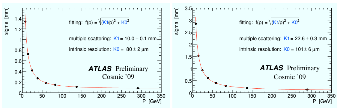
Figure 3: The track sagitta resolution measured inside the large (left plot) and inside the small (right plot) barrel sectors of the Muon Spectrometer as a function of the muon momentum.
