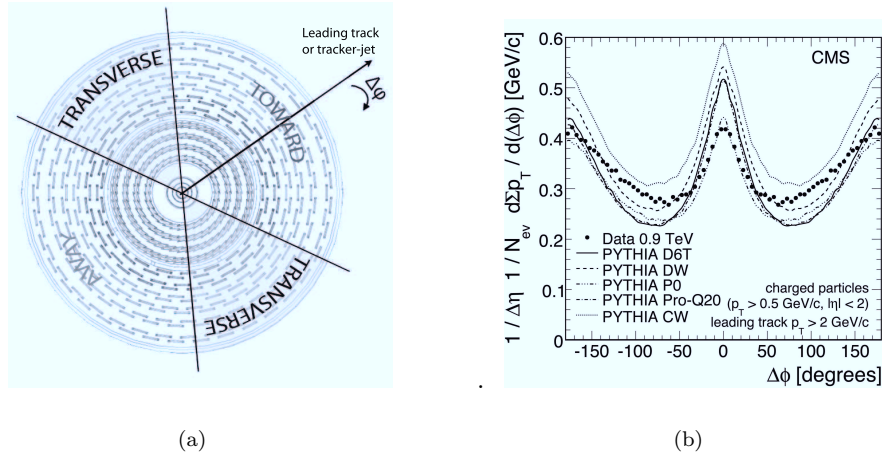
Figure 1: Representation of the three regions in the the x - y view of the CMS tracker (a). Average scalar p_T sum of tracks with p_T > 0.5 GeV/c and |\eta| < 2 per unit of pseudorapidity and per radian, as a function of \Delta\phi ; the leading track is excluded (b).
