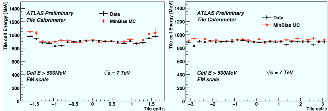
Figure 3: Tile calorimeter cell response uniformity as a function of pseudorapidity (left) and azimuthal angle (right) for 7 TeV collision and MC events.
