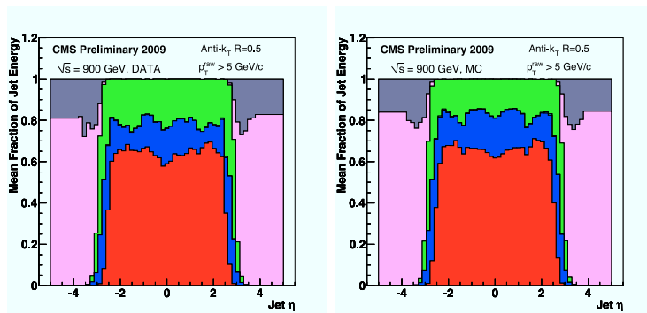
Figure 3: Reconstructed jet energy fractions as a function of pseudorapidity in the data (left), and in the simulation (right). From bottom to top in the central region: charged hadrons, photons, electrons (less than 1%), and neutral hadrons. In the forward region: hadronic deposits, electromagnetic deposits.
