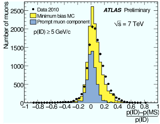
Figure 4: Efficiency of the combined reconstruction relative to the segment and calorimeter tagged muons. Figure 5: Relative difference between the inner detector and stand-alone muon momentum.
