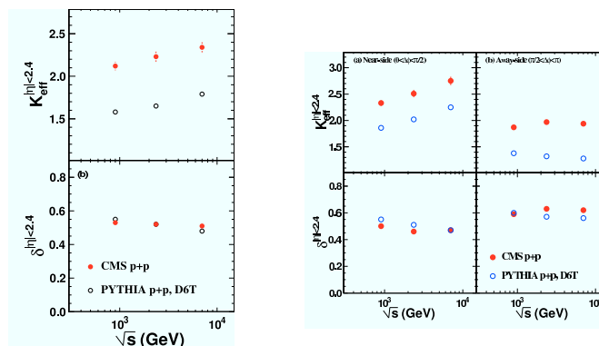
Figure 3: The two parameters K_{\text{eff}} and \delta determined from a fit to the CMS data at the three c.m. energies. The left figure indicates the result over the whole \Delta\phi range, while the right one is the result for the near- and away-side. The error bars indicate the systematic uncertainties, which are due to the tracking and event selection efficiencies and the model dependence of the corrections.
