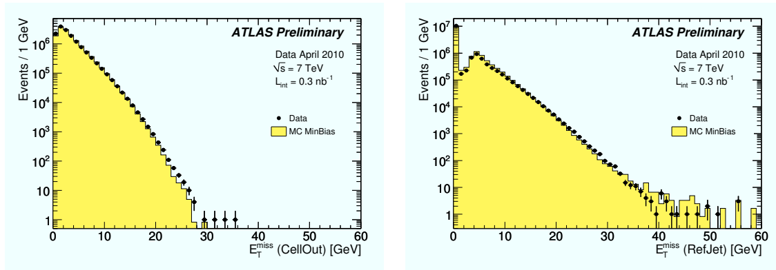
Figure 4: Distribution of E_T^{\text{miss}} computed with cells from topological clusters not in reconstructed objects (CellOut) (left) and distribution of E_T^{\text{miss}} computed with cells from topological clusters in Jets (RefJet) (right) for data (dots) and Monte Carlo simulation (histograms). The number of events in Monte Carlo simulation are normalized to the number of events in data.
