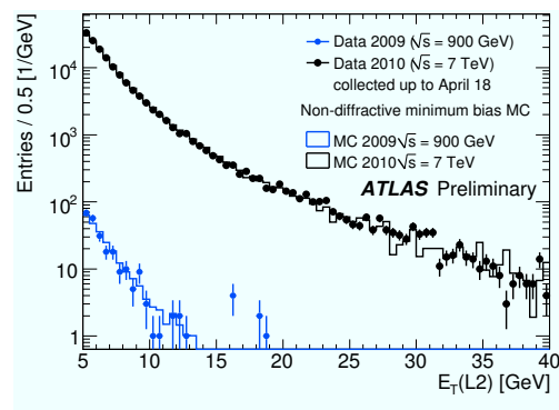
Figure 2: E_T spectrum of reconstructed clusters for data collected with 900 GeV and 7 TeV collisions. A comparison with a minimum bias MC is also shown.
