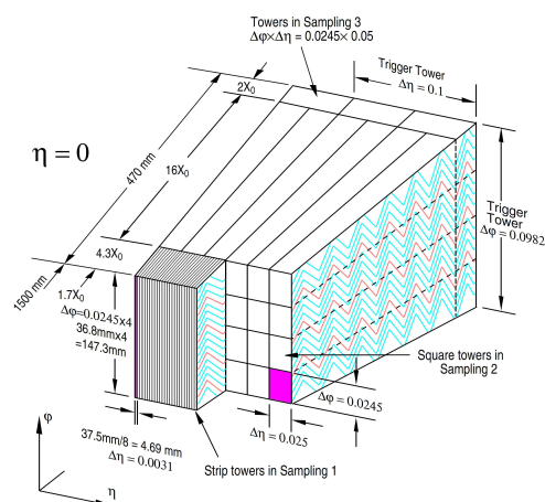
Figure 2: Readout granularity of the EM calorimeter.
