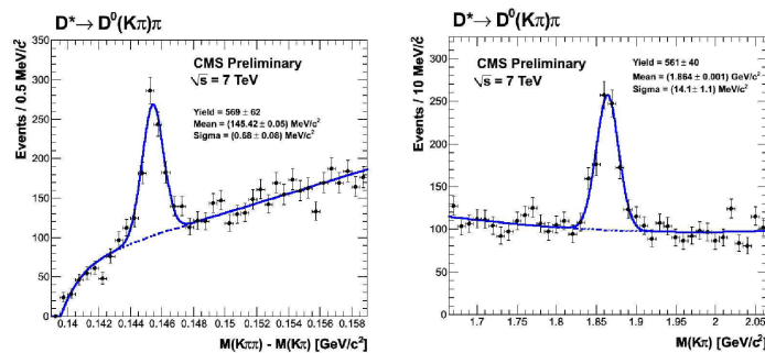
Figure 3: Distribution of the difference between the invariant masses of the K\pi\pi and K\pi systems (left) and of the reconstructed invariant mass of the K\pi system (right). The error bars are presenting only the statistical uncertainty.
