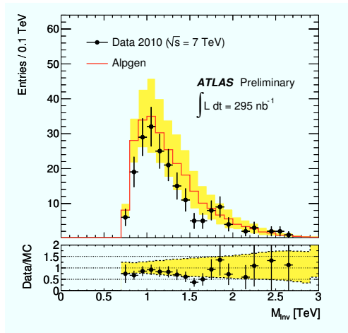
Figure 2: Invariant mass distribution for events with \sum p_T > 700 GeV. The solid dots are the data and the histogram is the rescaled background prediction using Alpgen simulation. The error band on the background is the total uncertainty: statistical (negligible) and systematic uncertainties added in quadrature.
