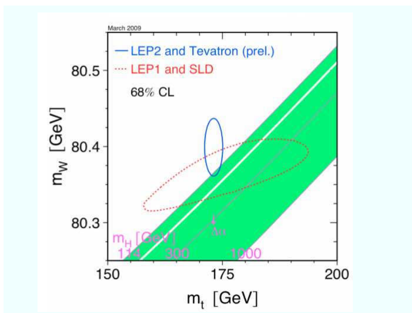
Figure 4: Current m_{top} and m_W measurements and their effect on the global electroweak fit and SM Higgs Boson.
