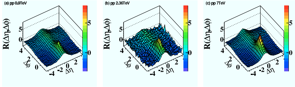
Figure 1: The 2-D two-particle correlation function R(\Delta\eta, \Delta\phi) for the CMS data at the three c.m. energies.
