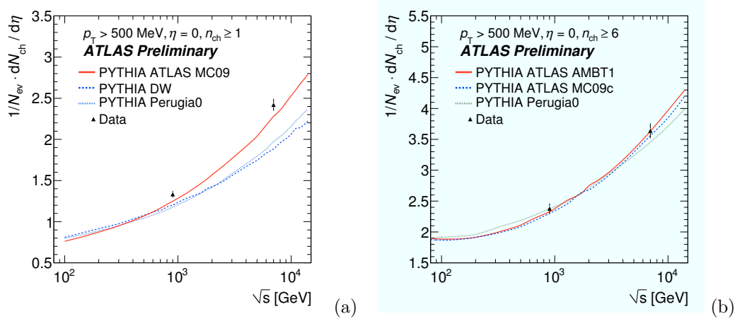
Figure 2: The average charged particle multiplicity per unit of rapidity for \eta = 0 for events with n_{ch} \geq 1 (a) [2] and in a diffractive limited phase-space n_{ch} \geq 6 (b) [3] within the kinematic range p_T \geq 500 MeV and |\eta| < 2.5 as a function of the centre of mass energy. In (b) the new ATLAS Minimum Bias Tune 1 is already shown.
