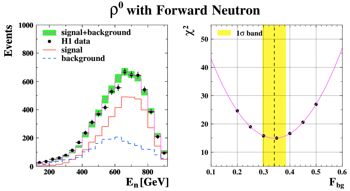
Figure 4: Signal to background decomposition in the selected data sample. On the left panel the distribution of the measured neutron energy, E_n , is shown together with the contributions from signal and background. On the right panel the \chi^2 dependence on the background fraction, F_{bg} , is shown. The shaded band represents the 1\sigma uncertainty around the optimal fit value of the F_{bg} , taking into account statistical errors, FNC calibration systematics and the uncertainty in proton dissociation background shape.
