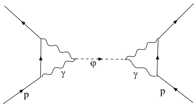
Figure 1: The Feynman diagram illustrating the ISL experiment’s sensitivity to a scalar-photon coupling.
