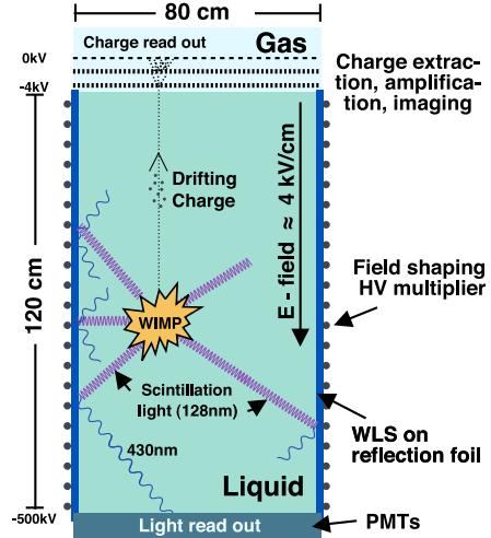
Figure 1: Conceptual design
