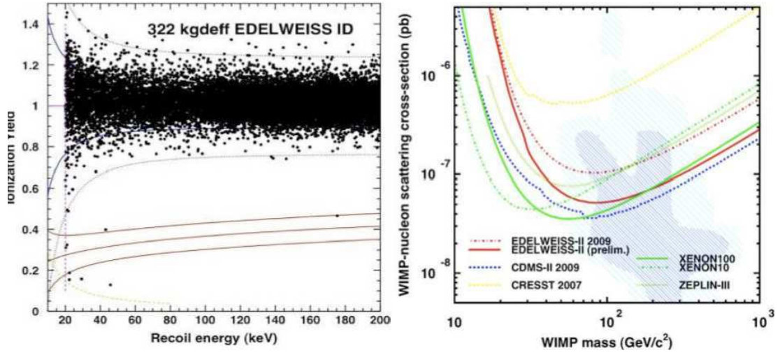
Figure 2: Left: Ionization yield vs energy for all fiducial interactions taking place in a WIMP search corresponding to a 322 kg \times days exposure. Right: The corresponding limit on the WIMP-nucleon cross-section (continuous red line) is compared to other experiments.
