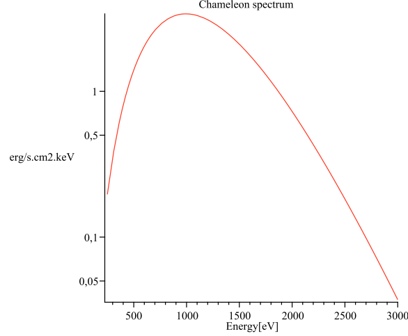
Figure 1: The energy spectrum of the emitted chameleons. Energies are expressed in eV and the spectrum in \text{erg/s.cm}^2.\text{keV} . The coupling is chosen to be M_\gamma = 10^{5.8} GeV and the magnetic field in the lower convection region is B=30 T which is the solar chameleon source. The integrated flux at the solar surface is 4 \text{ erg} \cdot \text{s}^{-1} \cdot \text{cm}^{-2} .
