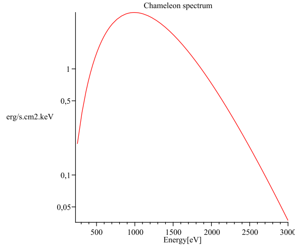
Figure 1: The energy spectrum of the emitted chameleons. Energies are expressed in eV and the spectrum in \text{erg/s.cm}^2\cdot\text{keV} . The coupling is chosen to be M_\gamma = 10^{5.8} GeV and the magnetic field in the lower convection region is B=30 T which is the solar chameleon source. The integrated flux at the solar surface is 4 \text{ erg} \cdot \text{s}^{-1} \cdot \text{cm}^{-2} .
