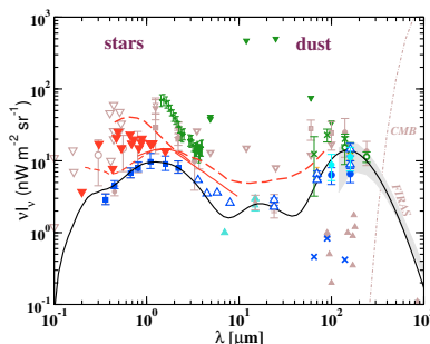
Figure 1: Extragalactic background light flux: data and limits (description and refs. see text). The black line is the lower limit EBL model [23] which gives a physically correct description of the lower limit data, including redshift evolution.
