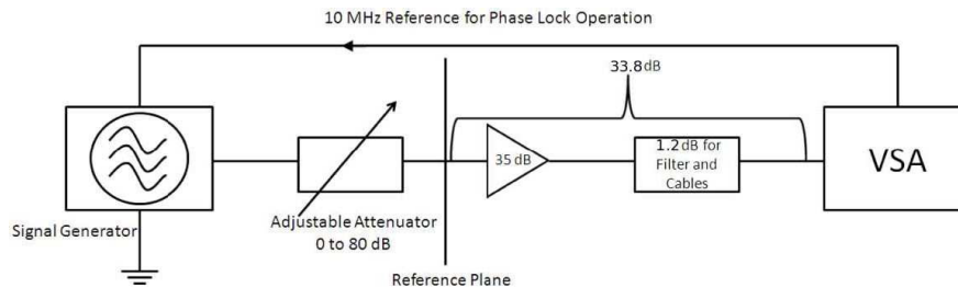
Figure 2: Measurment scheme [4]
