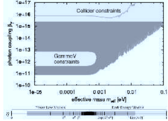
Figure 2: (a) The exclusion region of the coupling normalized to the Planck mass to photons versus the effective chameleon masses published for the GammeV reconfiguration (small region) and the results from GammeV-CHASE.
