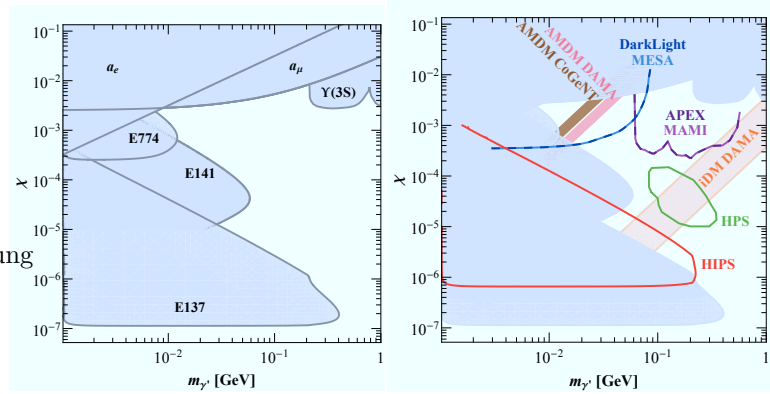
Figure 2: Exclusion regions ( left ) as well as projected sensitivities and phenomenological motivations ( right ) for the hidden photon. Dedicated proposals are being developed at DESY (HIPS, see also [22]), JLab (APEX [23, 24], HPS [25], DarkLight [21, 26]), and Mainz (MAMI, MESA [27]), with complementary sensitivities (cf. lines in Fig. 2, right).
