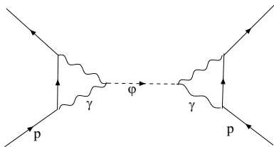
Figure 1: The feynmann diagram illustrating the ISL experiment’s sensitivity to a scalar-photon coupling.
