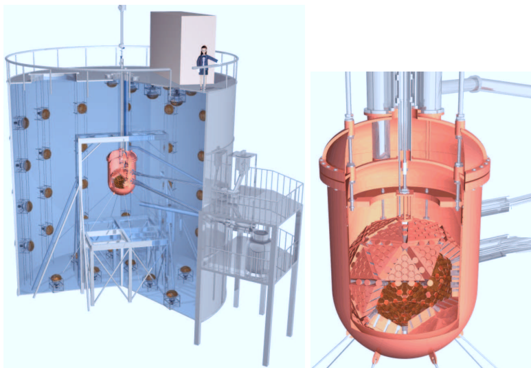
Figure 1: The water tank is used for the radiation shield (Left). The size of the tank is \phi 10 mm \times 10 m, the detector was installed in the center of it and 20 inch PMTs in the water will be used for the active veto for the cosmic ray events. 850 kg of liquid xenon will be surrounded by 642 ultra low radioactive PMTs. (Right) The double wall detector vessel made of the OFHC is about 1.2 m in inner diameter to hold liquid xenon with the vacuum insulation. The average radius of liquid xenon is about 40 cm.
