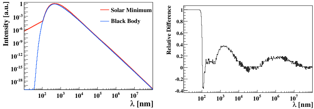
Figure 3: (( Left ) The approximated solar radiation spectrum during solar minimum (red line) and the black body spectrum for T=5800 K (blue line). ( Right ) The normalized relative difference between the two spectra can be used to unravel non-thermal contributions, whatever their origin. The residuals below \sim 100 nm correspond to the hot corona excess. Residuals at \sim 10^6 nm might be a contamination of the CMB radiation, though the peak appears too broad towards shorter wavelengths to be eventually explained exclusively by CMB (either directly or reflected from the Sun). The origin of the excess around \sim 2000 – 3000 nm is real, but it is not yet identified. (Courtesy Marlene DiMarco/ UCAR Office of Education and Outreach/2009.)
