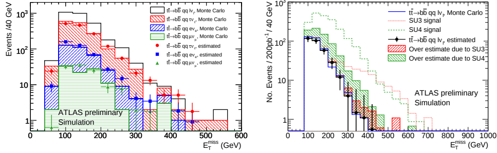
Figure 2: Left: E_T^{\text{miss}} distribution of t\bar{t} \rightarrow b\bar{b}l\nu q\bar{q} events (open histogram) and fractions of events with a tau lepton (left hatching), a lost electron (right hatching) and a lost muon (horizontal hatching), compared to the estimate of these fractions from the data-like sample. Right: E_T^{\text{miss}} distribution of t\bar{t} \rightarrow b\bar{b}l\nu q\bar{q} from MC prediction and from data-driven estimate with and without the presence of a SUSY signal with 200 \text{ pb}^{-1} at 10 TeV (SU4 is a mSUGRA benchmark point with 400 GeV squark and gluino masses).
