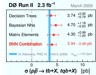
Figure 3: Summary of the measured cross sections compared to theoretical predictions.
