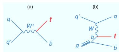
Figure 1: Feynman diagrams for s-channel (a) and t-channel (b) single top production.
