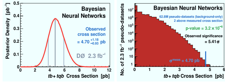
Figure 2: (Left)Posterior density distribution (Right)Cross section distributions on the pseudodatasets for BNN method.
