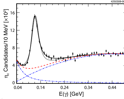
Figure 3: Fits to the photon spectrum in exclusive J/\psi \rightarrow \gamma\eta_c decays using relativistic Breit-Wigner (dotted) and modified (solid) signal line shapes convolved with a 4.8 MeV wide resolution function.
