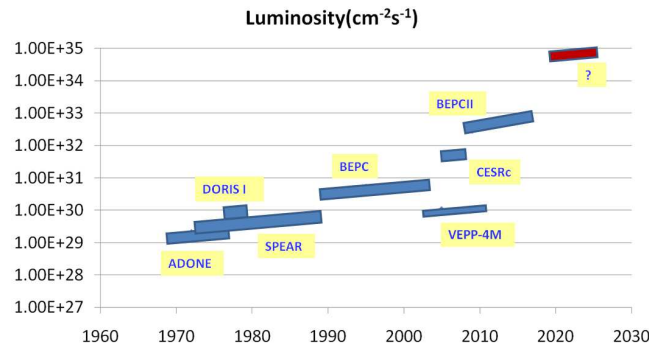
Figure 1: A history of accelerators running for tau-charm physics.
