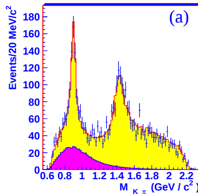
Figure 5: The observed \kappa^\pm signal at BESIII from an invariant mass spectrum of K^\pm \pi^0 . Shaded area are \kappa signals.
