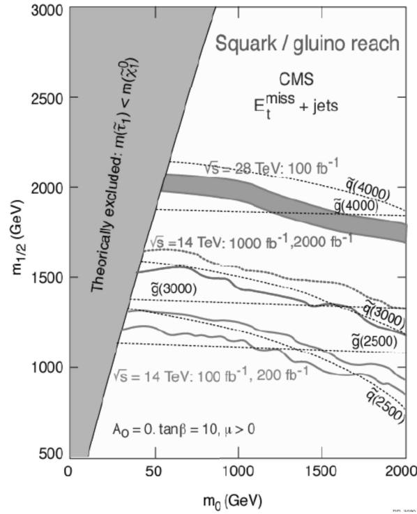
Figure 2: LHC SUSY mass reach for different luminosity and energy scenarios
