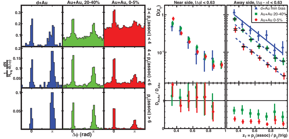
Figure 7: (colour online) left: Per-trigger yields of associated hadrons as a function of relative azimuthal angle for a trigger of p_T > 8 \text{ GeV}/c for d+Au, semi-central Au+Au and central Au+Au at different values of p_T of the associated hadrons. right: Per-trigger yields of correlated hadrons as a function of the momentum fraction z_T (definition see text) for the near side (left) and for the away side (right). The bottom panels show ratios of the upper distributions for Au+Au collisions to those for d+Au. (From[28])
