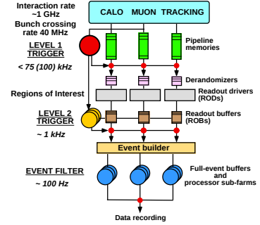
Figure 2: Schematic view of the ATLAS trigger and DAQ systems.
