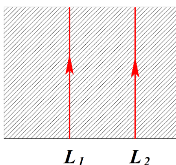
Figure 4. In the presence of surface operator and/or Omega-background line operators do not commute.
