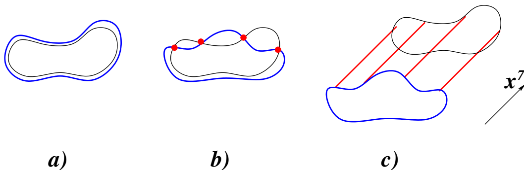
Figure 1. An M5'-brane wrapped on the curve C can be perturbed to a curve \tilde{C} which meets C at finitely many points u_i . Then, separating the five-branes on C and \tilde{C} along the x^7 direction results in creation of M2-branes (shown in red).
