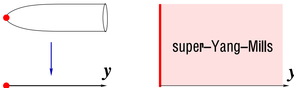
Figure 3. The six-dimensional (2,0) theory with a codimension-2 defect at the tip of the cigar reduces to 5d super-Yang-Mills theory with a non-trivial boundary condition.
