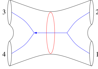
Figure 5. Pants decomposition of four-holed sphere with a numbering of boundary components.
