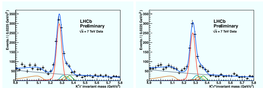
Figure 2: Invariant mass distributions for K^+\pi^- (left) and for K^-\pi^+ (right).
