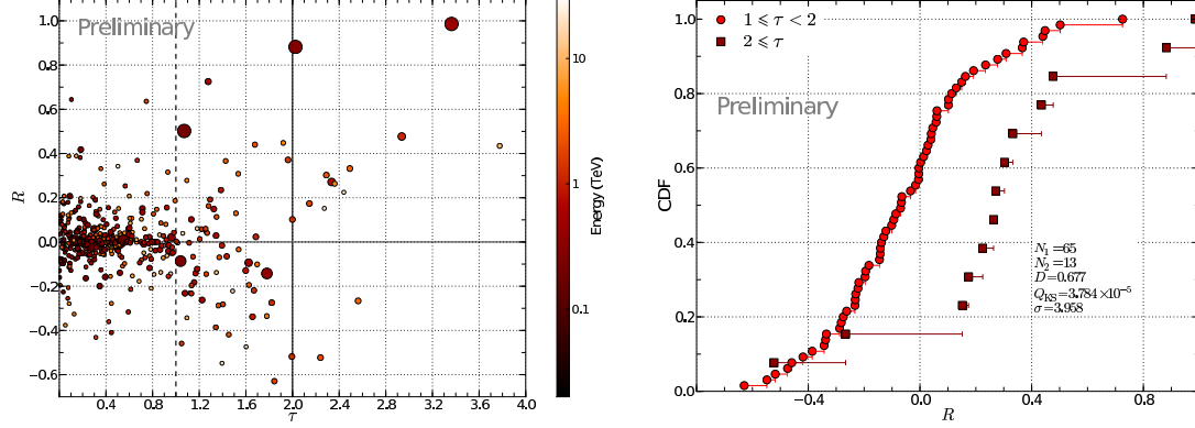
Figure 2: Result of the KS-test. Left Panel: The Ratios R plotted against the Optical depth \tau_{\gamma\gamma} . The size of the markers is proportional to the redshift while the color encodes the corresponding energy of each data point. Right panel: CDFs of \mathcal{S}_{\text{thin}} and \mathcal{S}_{\text{thick}} .
