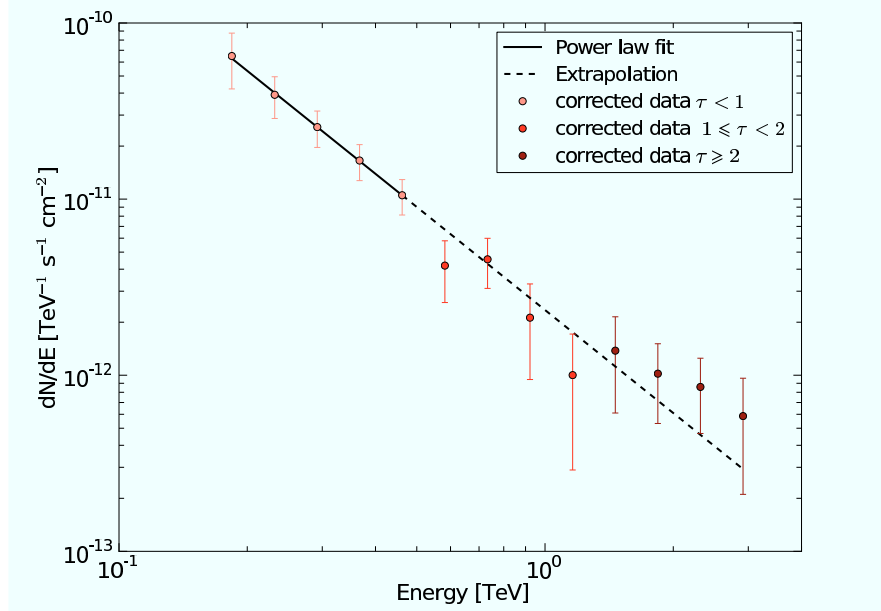
Figure 1: The spectrum of 1ES 1101-232 measured with H.E.S.S. [14] with 1\sigma statistical errors on the flux. The first five points correspond to a \tau_{\gamma\gamma} value smaller than one and thus enter into the power-law fit. The fit itself is shown as a black solid line. The fit is extrapolated to all other points (dashed line) and the ratios R_i are calculated according to Eq. 2. The ratios of the red points enter \mathcal{S}_{\text{thin}} while the ratios of the dark red points contribute to \mathcal{S}_{\text{thick}} , see Eq. 3 and 4.
