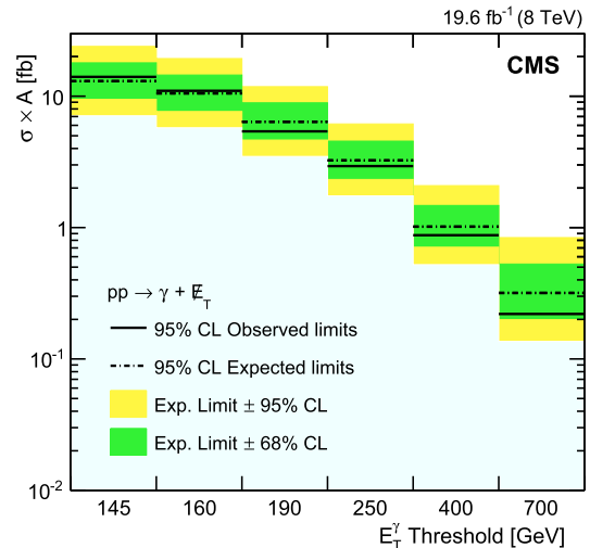
Fig. 2. Upper limits at 95% confidence level (CL) on the product of cross section and acceptance as a function of the E_T^\gamma threshold ( >145 GeV) for the photon and \cancel{E}_T final state.
