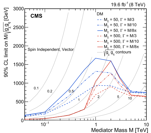
Fig. 4. Observed limits on the SM-DM interaction mediator mass divided by coupling, M/\sqrt{g_\chi g_q} , as a function of the mediator mass M , assuming vector interactions, for DM particle masses of 50 GeV and 500 GeV. The width, \Gamma , of the mediator is varied between M/8\pi and M/3 . The dotted lines show contours of constant coupling.
