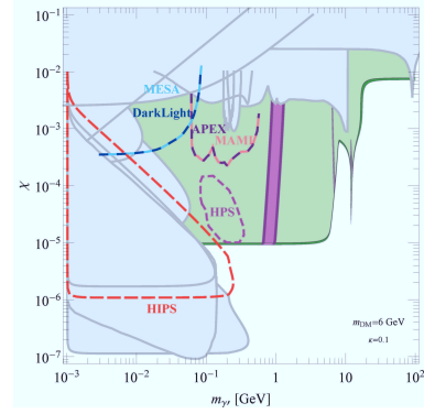
Figure 2: Toy model HS with relic abundance (green) and CoGeNT region (purple) for the Dirac fermion DM.
