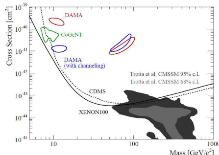
Figure 2: Exclusion plots for spin independent WIMP-nucleon interactions. The current limits are the curves around 10^{-43} \text{ cm}^2 , given by XENON100 (solid,[8]) and CDMS II (dashed,[9]). The projected sensitivity for XENON100 is one order of magnitude lower. The shaded regions are theoretical expectations of CMSSM.
