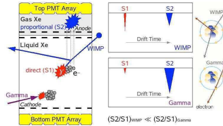
Figure 1: Principle of a two-phase liquid xenon TPC. A particle generates primary scintillation light (S1) and ionization electrons. These are drifted upwards with the field and detected via secondary scintillation light in the gas phase (S2). The S2 hit pattern (xy) and the drift time (z) give complete information for the position of events. Additionally, the ratio S2/S1 allows event discrimination between nuclear recoils (WIMPs, neutrons) and electron recoils ( \gamma , \beta ).
