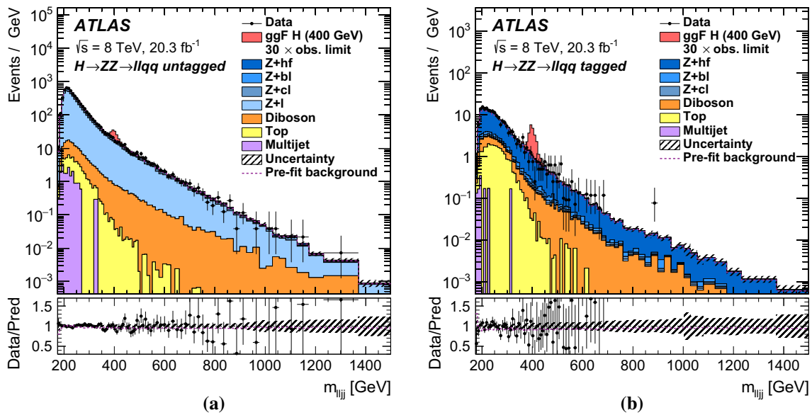
Fig. 3 The distributions used in the likelihood fit of the invariant mass of dilepton + dijet system m_{\ell\ell jj} for the H \rightarrow ZZ \rightarrow \ell^+ \ell^- q \bar{q} search in the a untagged and b tagged resolved ggF subchannels. The dashed line shows the total background used as input to the fit. The simulated signal
