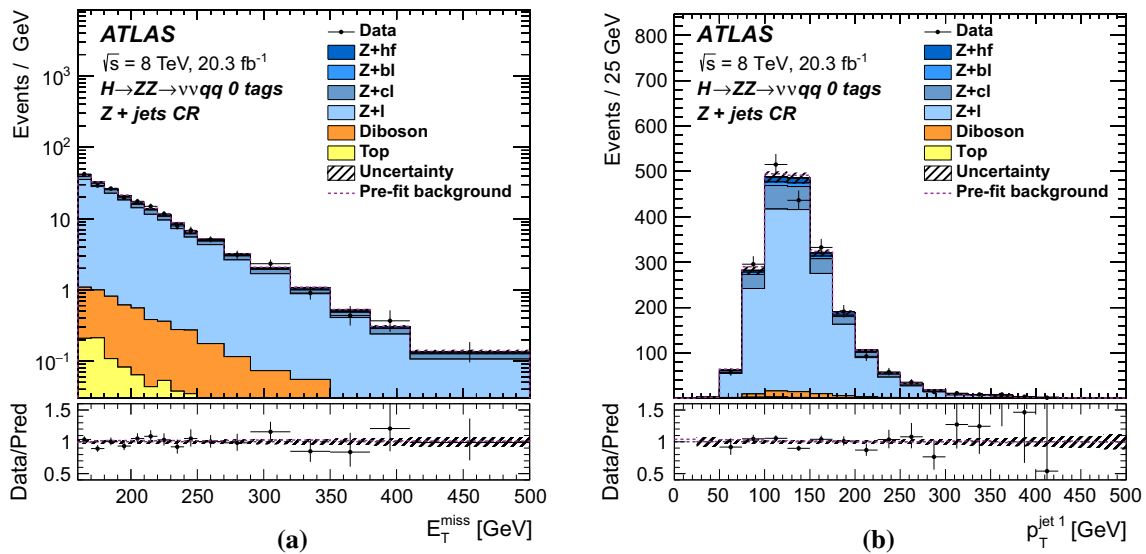
Fig. 10 The distributions of a missing transverse momentum E_T^{\text{miss}} and b leading-jet p_T from the untagged ( Z \rightarrow \mu\mu ) + jets control sample of the H \rightarrow ZZ \rightarrow \nu\nu q\bar{q} search. The dashed line shows the total
