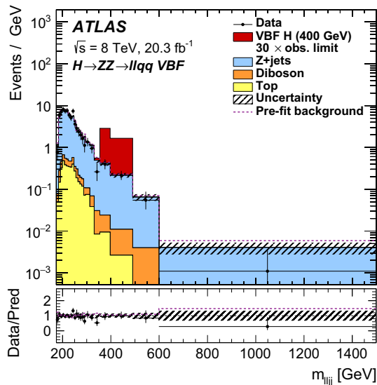
Fig. 6 The distribution of m_{\ell\ell jj} used in the likelihood fit for the H \rightarrow ZZ \rightarrow \ell^+\ell^-q\bar{q} search in the VBF channel. The dashed line shows the total background used as input to the fit. The simulated signal is normalized to a cross-section corresponding to 30 times the observed limit given in Sect. 11. The contribution labelled as ‘Top’ includes both the t\bar{t} and single-top processes. The bottom pane shows the ratio of the observed data to the predicted background
