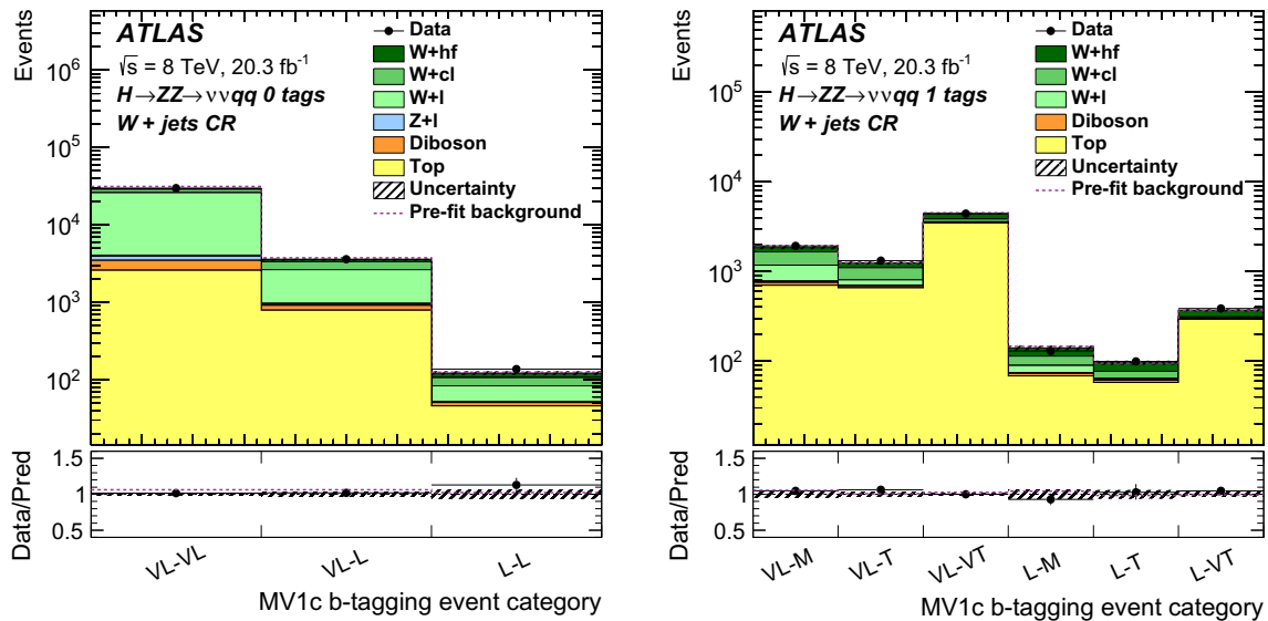
Fig. 17 The distribution of the MV1c b -tagging event categories, based on the two signal jets, in the W + \text{jets} a 0- b -tag and b 1- b -tag control regions of the H \rightarrow ZZ \rightarrow \nu \bar{\nu} q \bar{q} search. The b -jet purity generally increases from left to right. The dashed line shows the total
