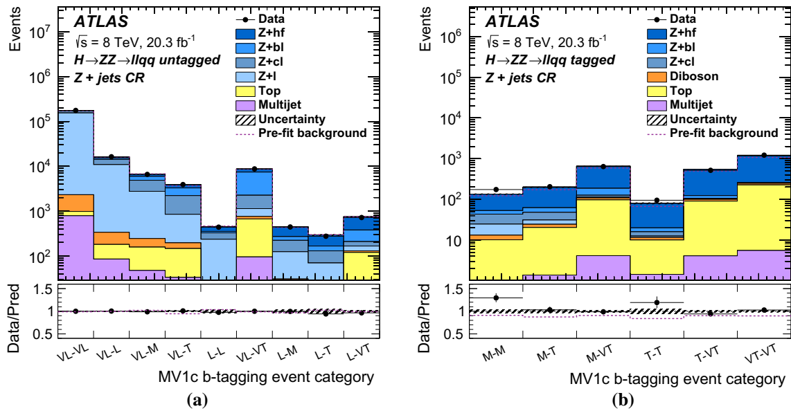
Fig. 16 The distribution of the MV1c b -tagging event categories, based on the two signal jets, in the Z + \text{jets} control region in the a untagged ggF and b tagged ggF channels of the H \rightarrow ZZ \rightarrow \ell^+ \ell^- q \bar{q} search. The b -jet purity generally increases from left to right. The dashed
