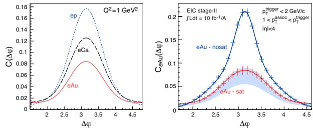
Figure 2: Saturation model [10] predictions of azimuthal angle difference ( \Delta\phi ) between two hadrons in ep , eCa , and eAu (left), and comparisons with calculations from conventional non-saturated model (right).
