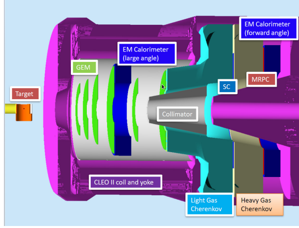
Figure 1: The experimental layout of the SoLID and polarized target in the proposed measurement. The subdetectors are labeled with colors corresponding to the detector regions.
