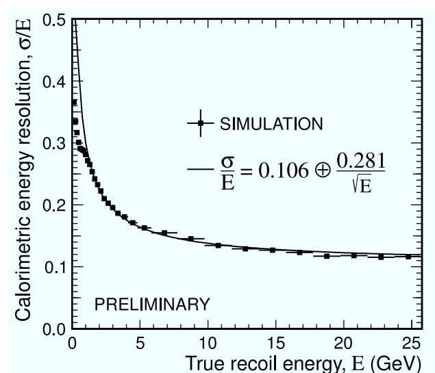
Figure 2: Calorimetric energy resolution vs. true recoil energy. The solid curve is the parametrized fit to the points.
