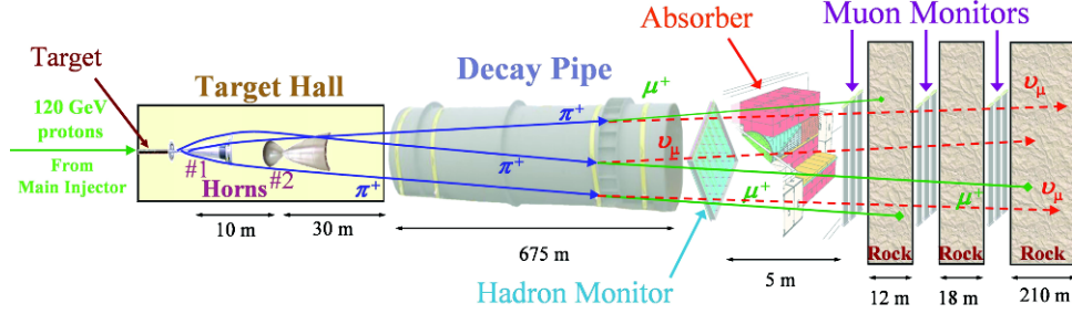
Figure 1: Diagram of the MINERνA beamline, showing the muon monitors and moveable magnetic horns.
