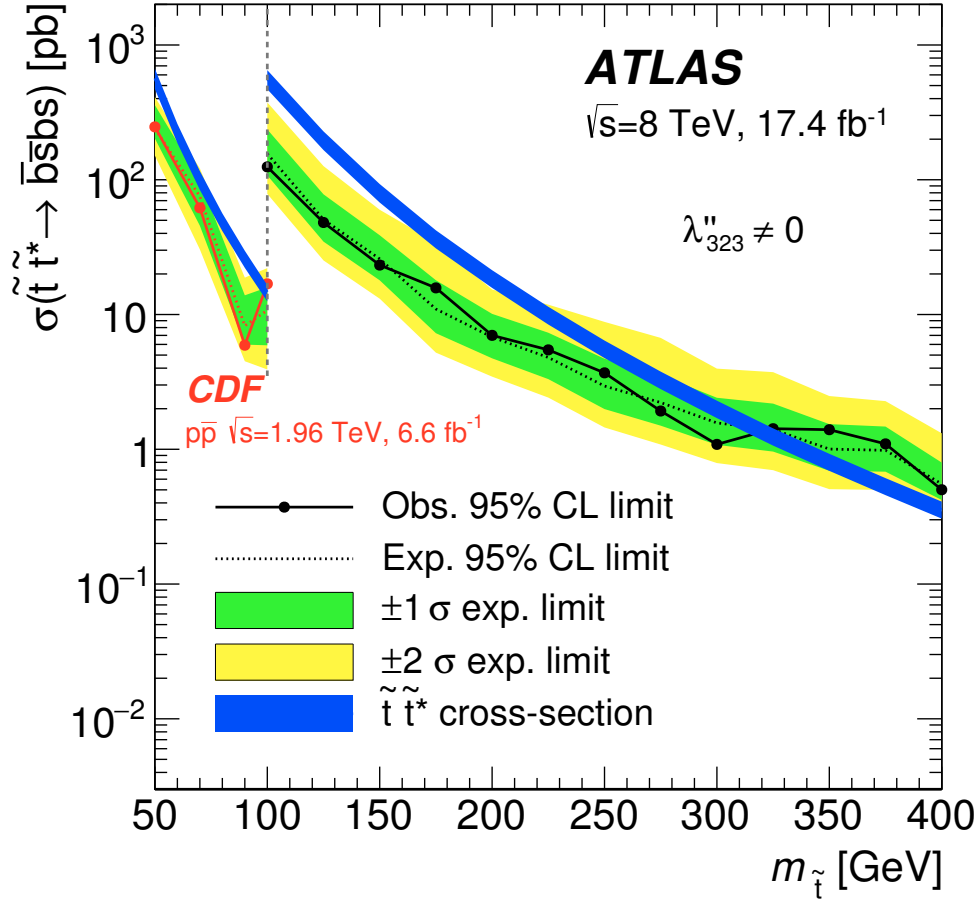
Figure 10: Observed and expected 95% CL upper limits on the stop pair production cross-section as function of the stop mass. The solid line with big round markers shows the observed limit, the dotted line shows the expected exclusion limit, and the green and yellow bands represent the uncertainties on this limit. Limits from the CDF Collaboration are shown in red for m_{\tilde{t}} \leq 100 GeV [40]. The blue line shows the theoretical signal cross-section and the blue band indicates the \pm 1\sigma variations due to theoretical uncertainties on the signal production cross-section given by renormalisation and factorisation scale and PDF uncertainties. For this search the cross-section is calculated at NLO+NLL, whereas in the CDF paper the cross-section was calculated at NLO only.
