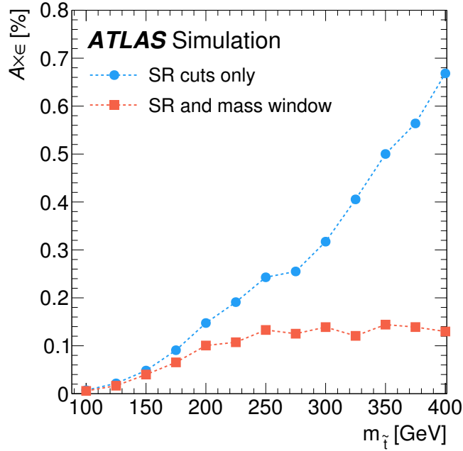
Figure 5: Total acceptance times efficiency ( A \times \epsilon ) of the SR cuts of Eq. (5), and SR cuts combined with the mass window selection in Table 1, as a function of m_{\tilde{t}} .
