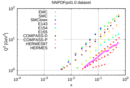
Figure 1: Experimental dataset after kinematic cuts for the NNPDFpol1.0 analysis.
