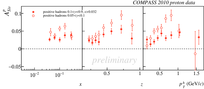
Figure 3: Sivers asymmetries of 2010 proton data as a function of x , z and p_T^h for 0.1 < y < 0.9 and 0.05 < y < 0.1 with x > 0.032 , positive hadrons only.
