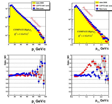
Figure 2: Data/MC agreement for different LEPTO tunings for longitudinal and transverse momenta of the first hadron.
