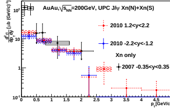
Figure 3: PHENIX 2010 dimuon (Red and Blue) and 2007 dielectron(black) UPC J/\psi \frac{d^2\sigma}{dp_T dy} . Dielectron distribution has significant 0 p_T peak, but same peak can't be find from dimuon distribution.
