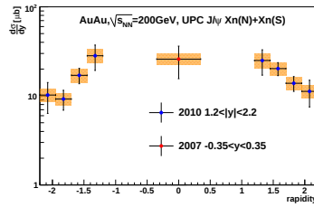
Figure 4: PHENIX 2010 RUN UPC J/\psi \frac{d\sigma}{dy} distribution
