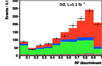
Figure 2: Multivariate discriminant.
