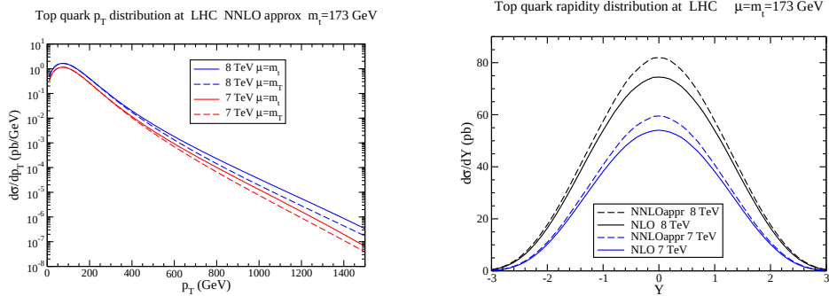
Figure 2: Top quark p_T (left) and rapidity (right) distributions at the LHC [ m_T = \sqrt{p_T^2 + m_t^2} ].
